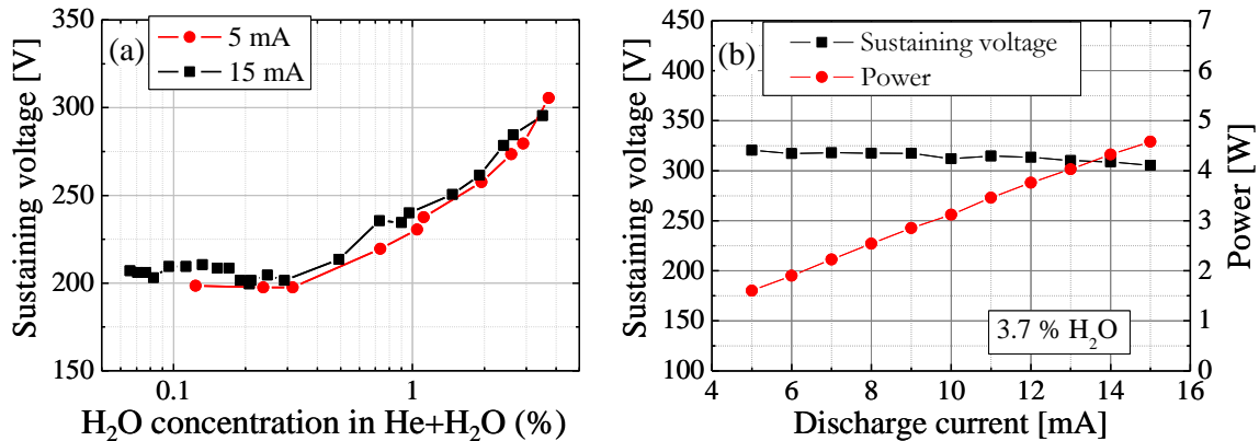
Fig. 2. Discharge characteristics: (a) sustaining voltage as a function of the H_2O concentration in He+H_2O and (b) sustaining voltage and input power as a function of discharge current for 3.7% H_2O .
