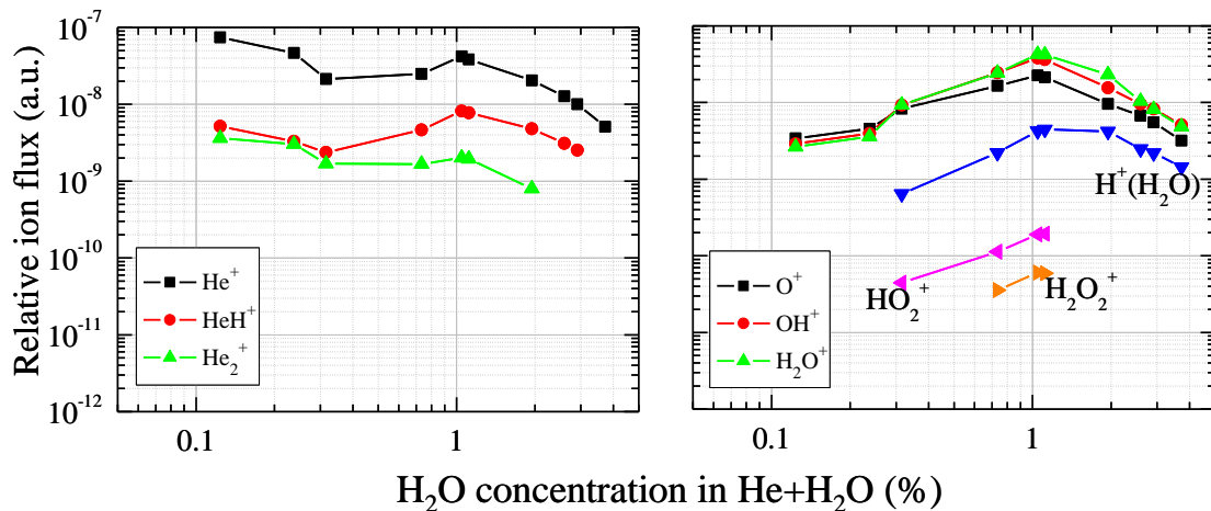
Fig. 5. Relative ion flux as a function of \text{H}_2\text{O} concentration in \text{He}+\text{H}_2\text{O} at a discharge current of 15 mA and sustaining voltage of 199 to 309 V.
