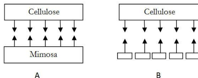
Fig. 11. Symmetric bonding diagram of cellulose and mimosa, A is more stable than B.
