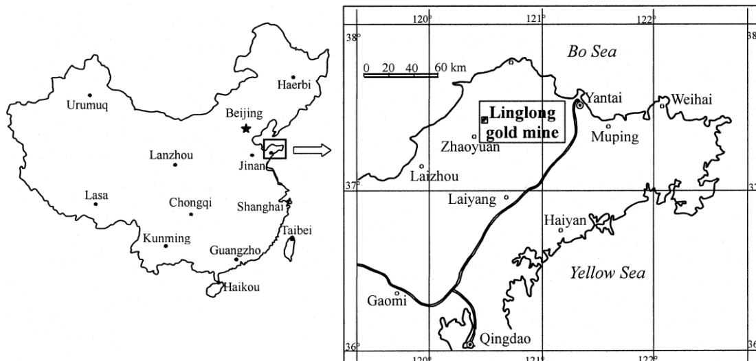
Fig. 2. Location of the Linglong gold mine.
